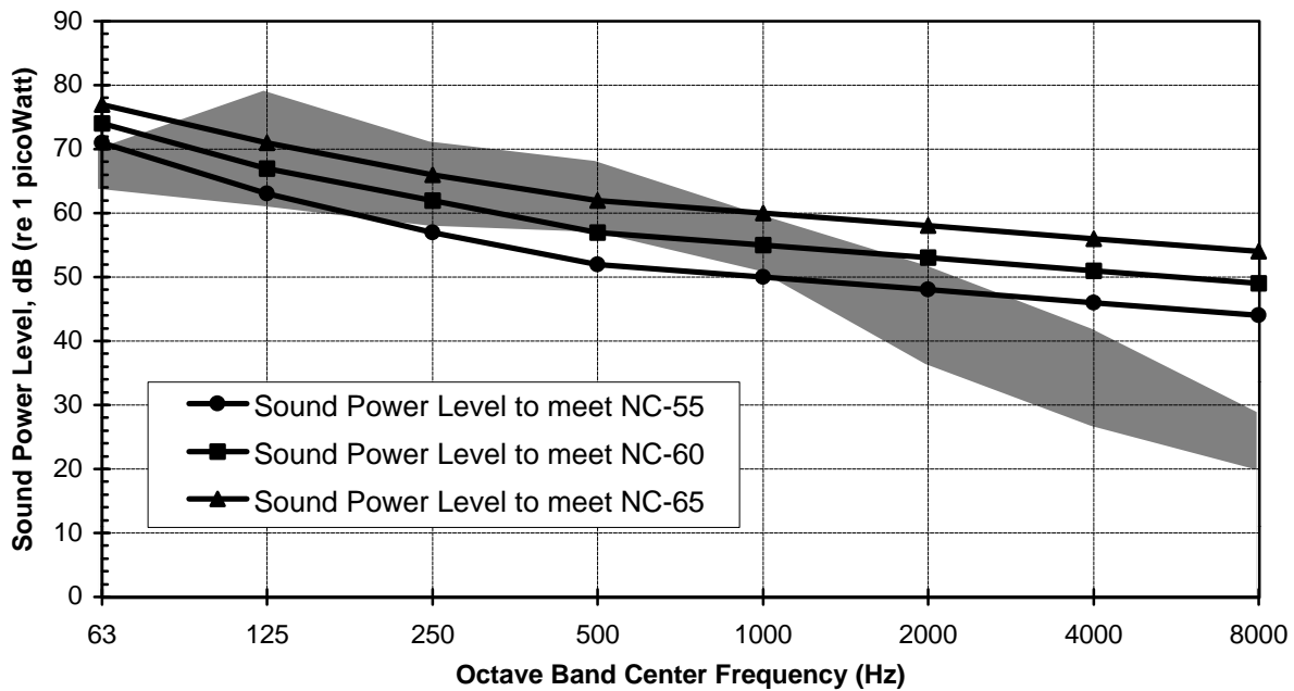
Figure 3. Range of measured FFU sound power levels for seven units running at 100 fpm versus requirements for 25% ceiling coverage.
