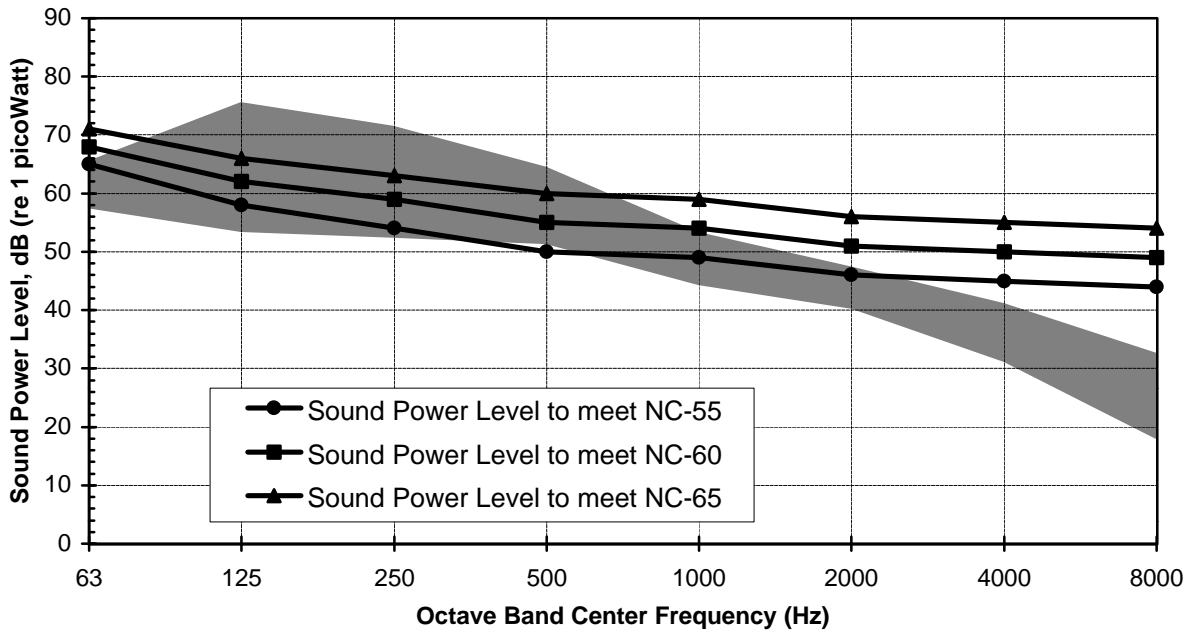
Figure 4. Range of measured FFU sound power levels for six units running at 75 fpm versus requirements for 100% ceiling coverage.
