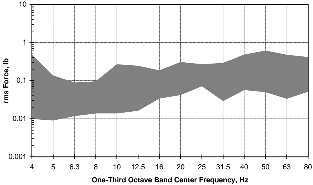
Figure 7. Range of calculated rms force for five FFU units running at 100 fpm based on rigid body motion.
