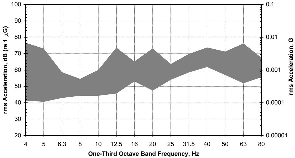
Figure 6. Range of measured FFU vertical rms acceleration amplitudes on five units running at 100 fpm
