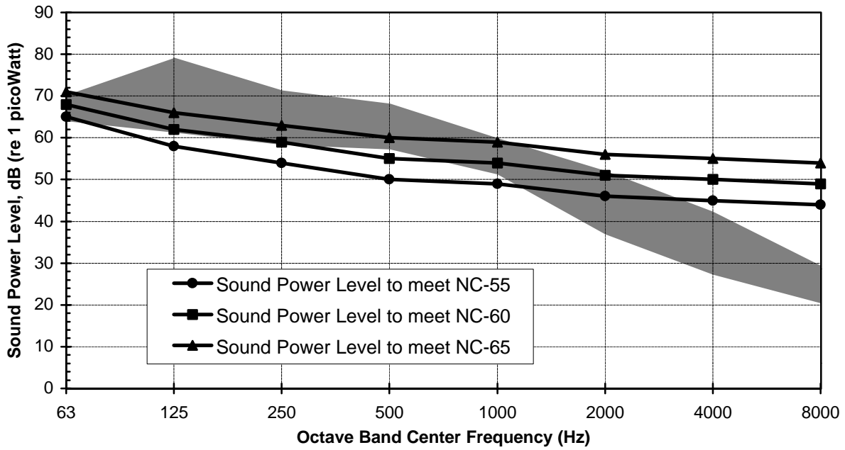
Figure 2. Range of measured FFU sound power levels for seven units running at 100 fpm versus requirements for 100% ceiling coverage.
