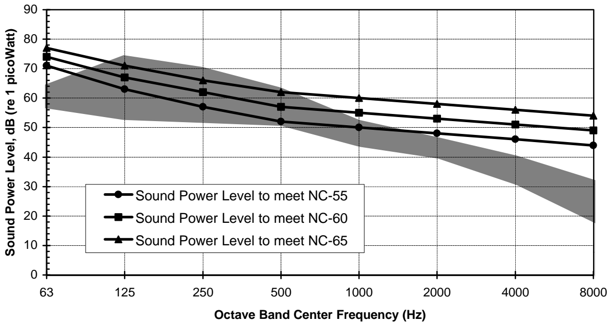
Figure 5. Range of measured FFU sound power levels for six units running at 75 fpm versus requirements for 25% ceiling coverage.
